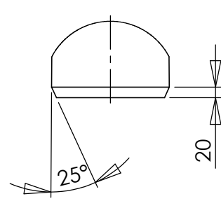
DETAIL C SCALE 1 : 10
